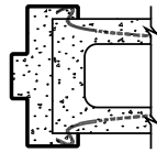
Wrap-around masonry
